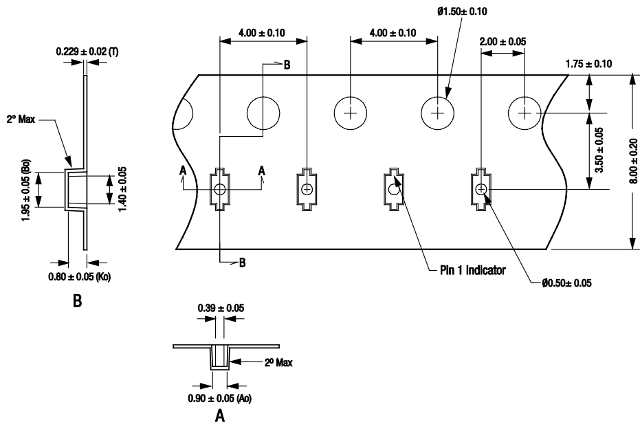
Figure 8. SC-79 Package Dimensions
